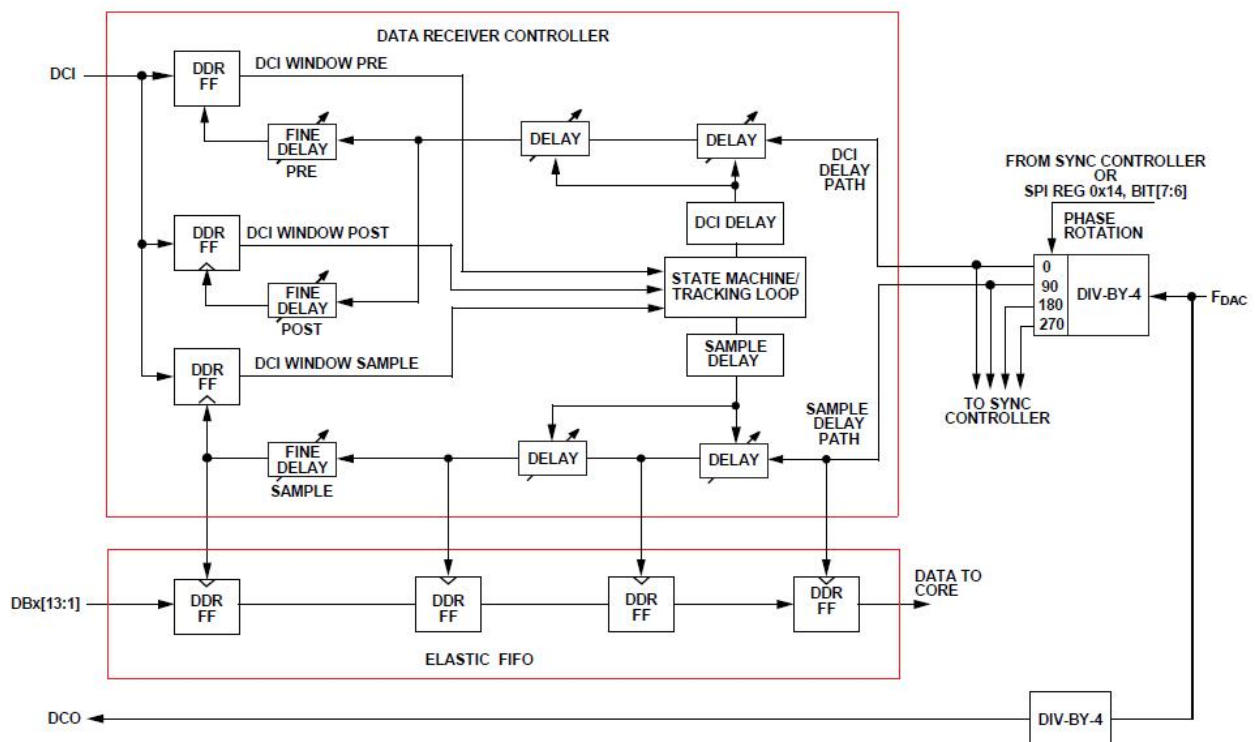
Figure 25. Top Level Diagram of the Data Receiver Controller
